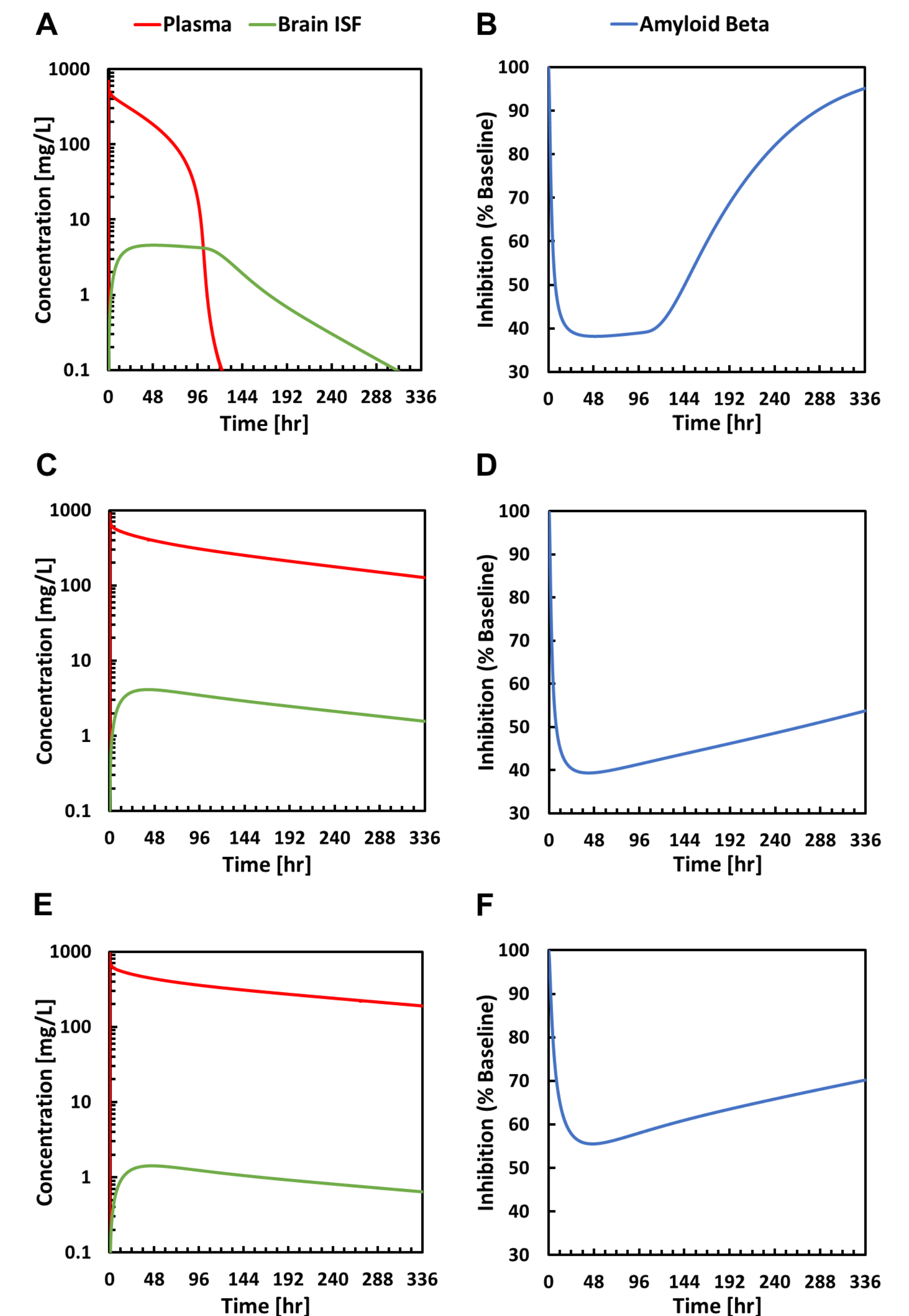
Figure 3. A, Plasma and brain ISF concentration when antibody-transferrin receptor k_D of 3nM. B, amyloid- \beta inhibition at 3nM k_D . C, Plasma and brain ISF concentration at k_D of 30,000nM. D, amyloid- \beta inhibition at 30,000nM k_D . E, Plasma and brain ISF concentration without Tfr binding. F, amyloid- \beta inhibition without Tfr binding.
